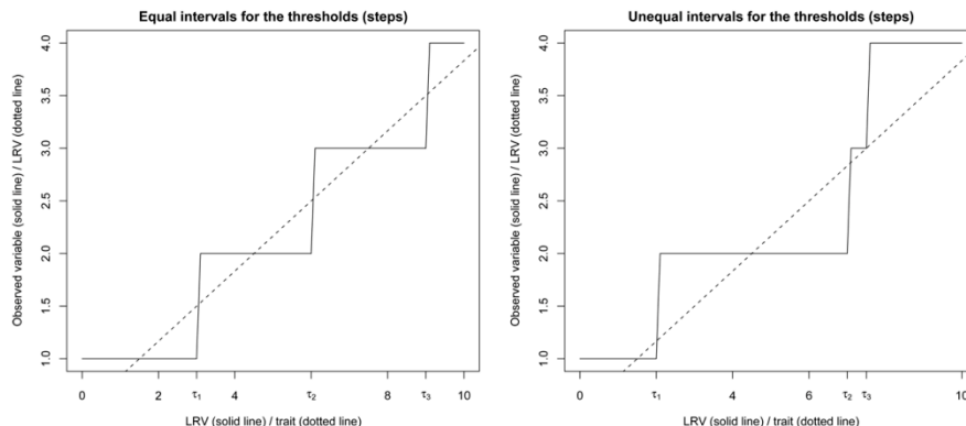
Figure 23.4. Two hypothetical step functions resulting from categorization. The solid lines plot the observed categorical variable as a function of the latent response variable (LRV). The diagonal dotted lines plot the expectation of the LRV as a function of the latent trait on the same scale. The thresholds used for categorization are denoted by the symbols \tau_1 , \tau_2 , and \tau_3 .
