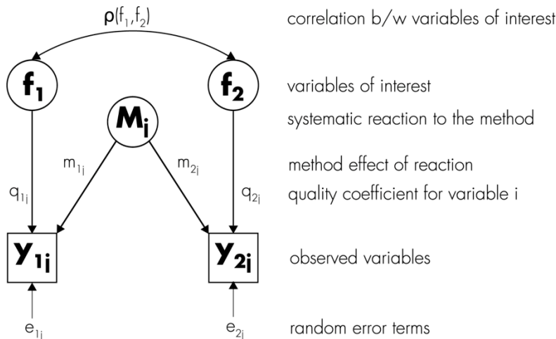
Figure 23.1. The Continuous Response Model Used in the MTMM Experiments
