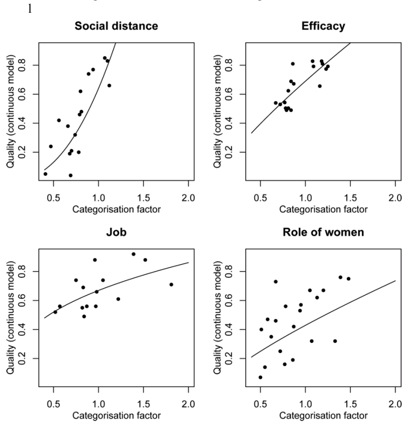
Figure 23.6. Scatterplot of the categorization factor ( c ) and the total quality of a measure ( q_{con}^2 ) by experiment. The prediction line of the model \ln(q^2) = \alpha + \beta \ln(c) , as estimated for each experiment separately, is also given. For the numerical estimates of these coefficients, please see the appendix.
