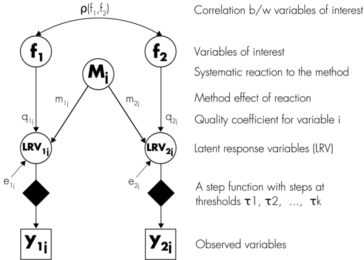
Figure 23.3. The Categorical Response Model Used in the MTMM Experiments
