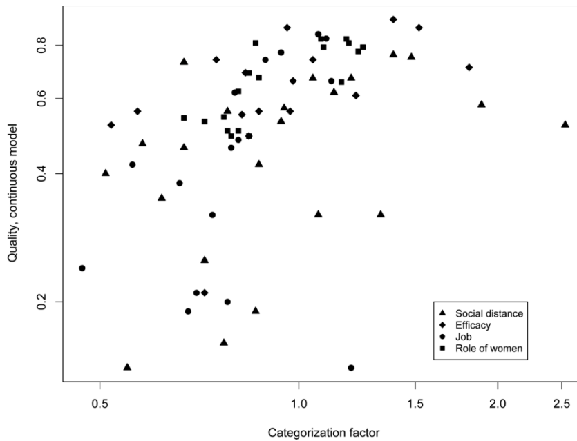
Figure 23.5. Scatterplot of the categorization factor ( c ) and the total quality of a measure ( q^2_{con} ) across the experiments. Note the log-log scales.
